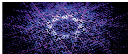
Condensed matter
